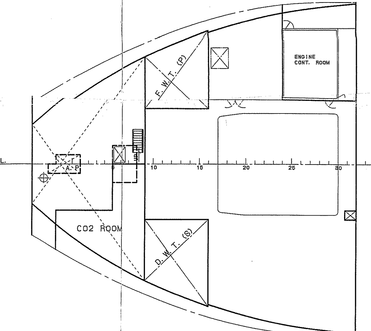
3RD DECK
