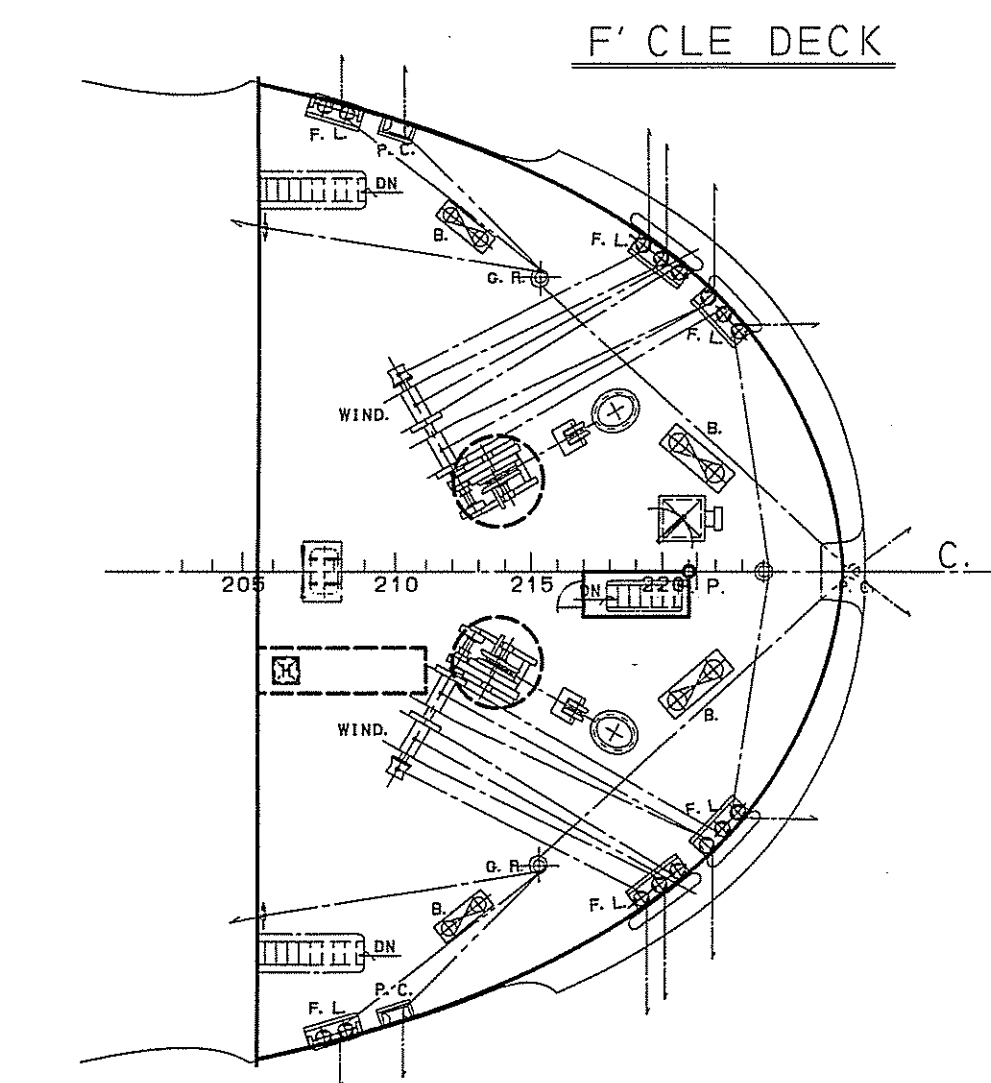
UPPER DECK
