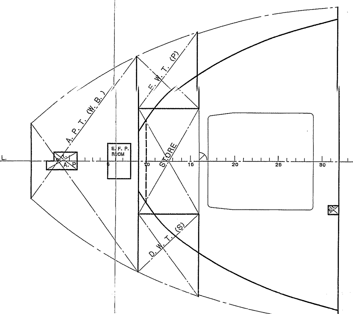
3RD DECK
