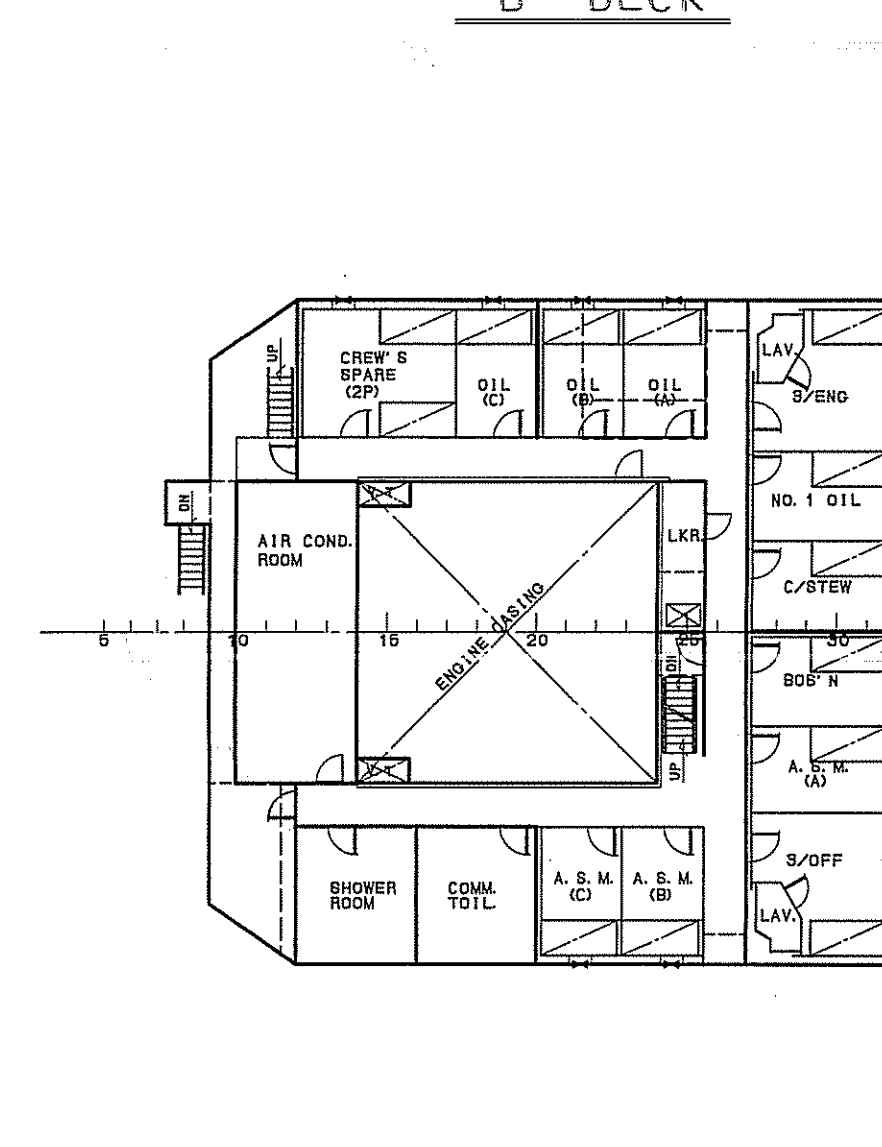
'B' DECK
