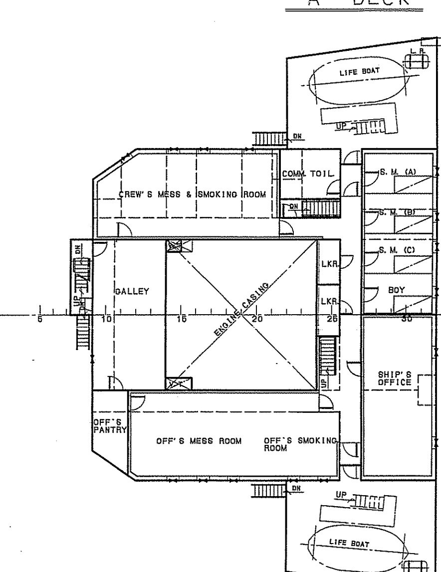
'A' DECK
