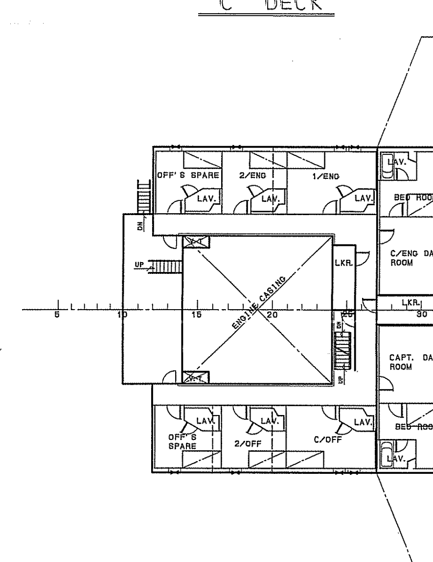
'C' DECK
